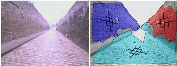
Figure 1: An example result of our algorithm. From such an image as this, we can detect planes and predict their 3D orientation, as shown on the right.
